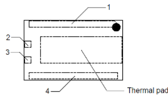
Package Outline
