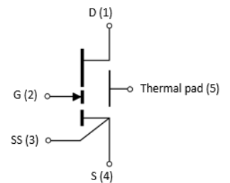
Circuit Symbol
